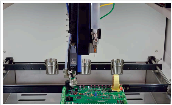
Adjustable Fixture
